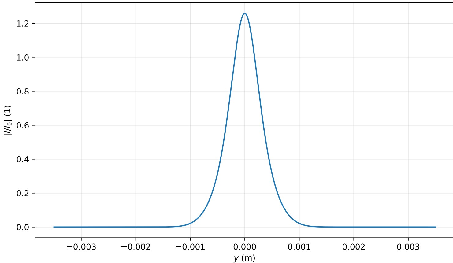
Intensity profile I(x=0, y, z=0.716)/I_0 , P_{in}=0.9P_{cr} , artificial time
